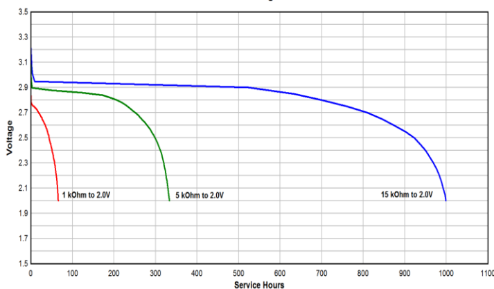
Continuous Discharge - Service Life
