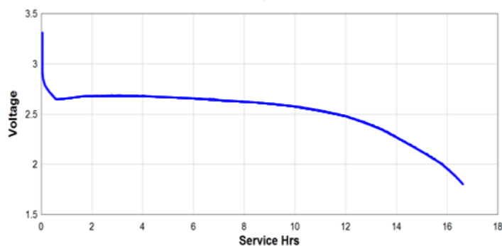
ANSI Key Fob Test 10 mA 5s/m, 24hd 1.8 New
