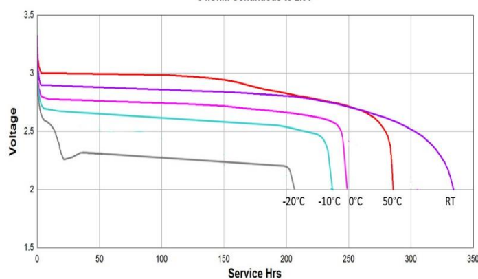
Temperature Discharge 5 kOhm Continuous to 2.0V
