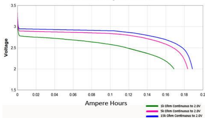
Continuous Discharge Characteristics
